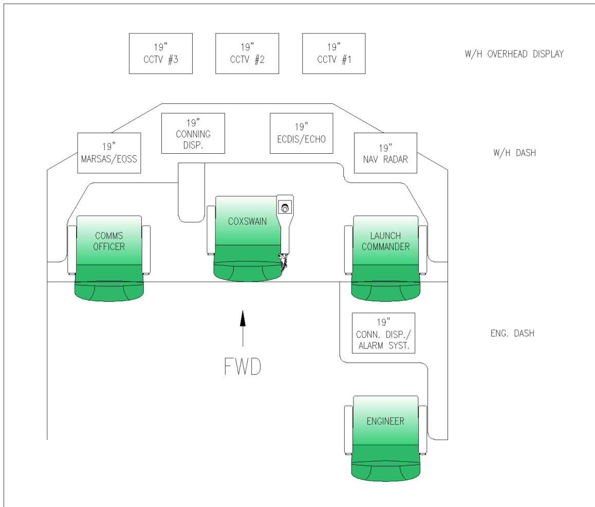
Figure 9.1 Navigation Station in the Wheelhouse
