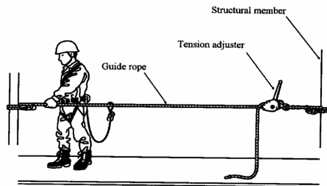
Figure 9: Horizontal Lifeline
